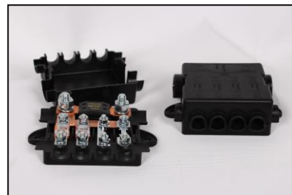
Combi Fuse Holder (Product codes: FH1005-A & FH1005-B)
